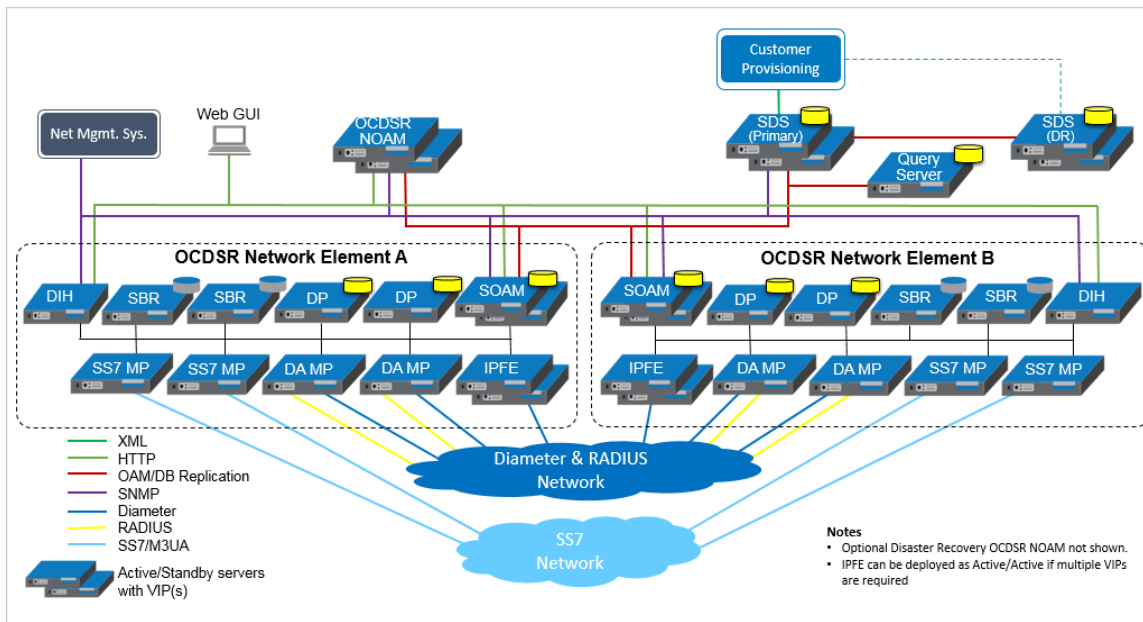
Figure 2. DSR System Architecture
